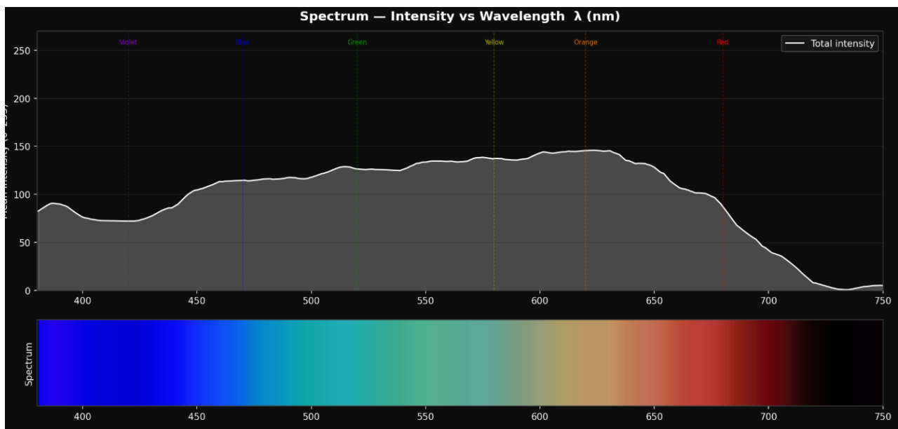
The composition of our Light Source: Intensity across the Visible Spectrum
